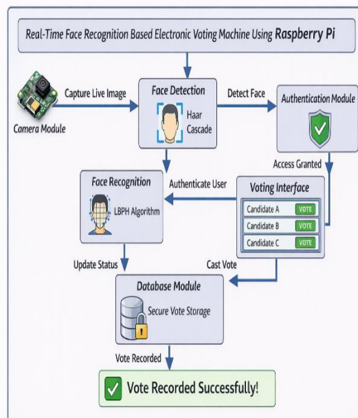
Fig.1 Proposed Architecture
