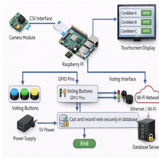
Fig.3 Proposed system hardware implementation
