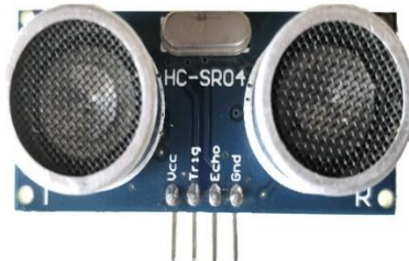
Fig 3.2 Ultrasonic Sensor
