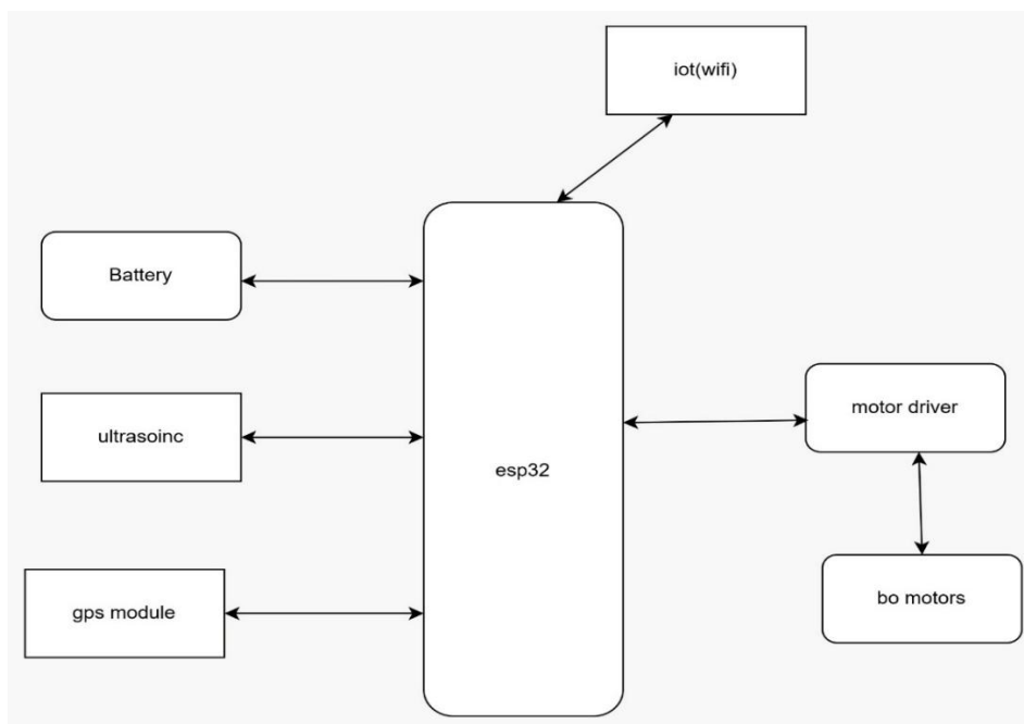
Fig 4 Block Diagram
