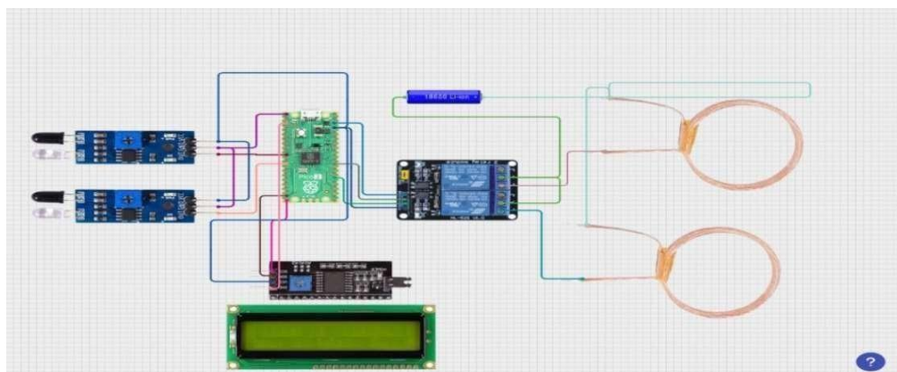
Fig 1: Circuit Diagram
