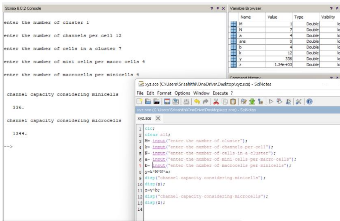
Fig. 1 Scilab code and result
