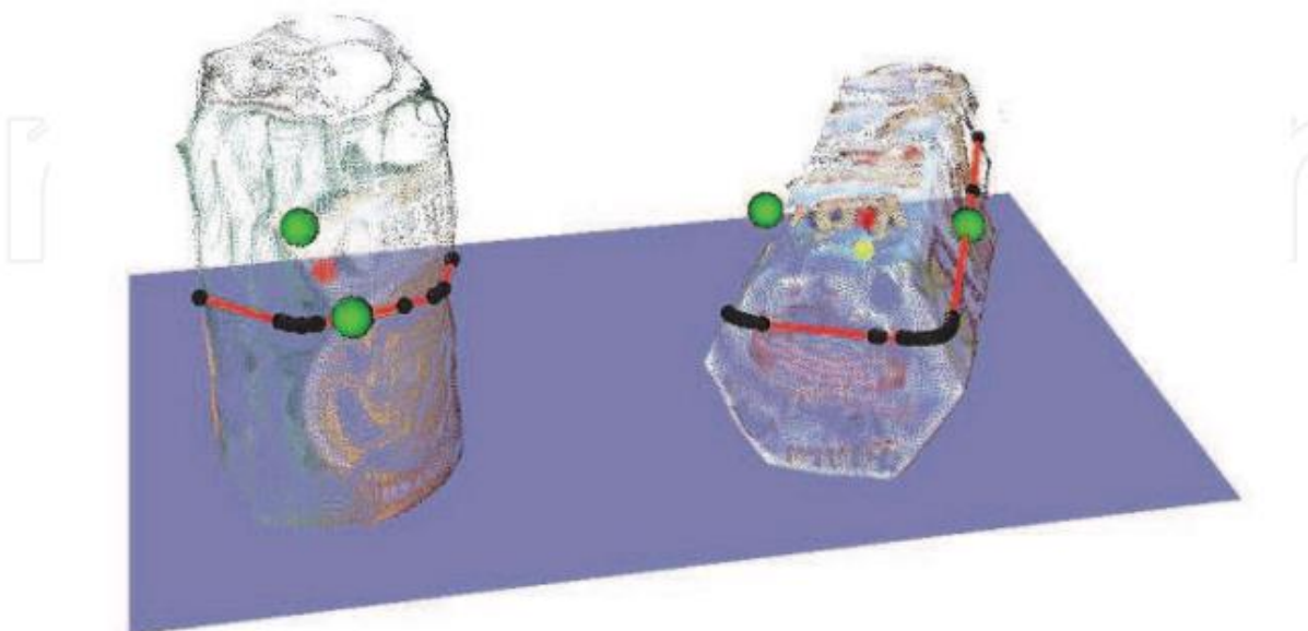
Fig. 7. Calculated grasping points (green) based on stereo data. The yellow points show the centre of mass of the objects. If, through the check of the 3D gripper no accurate grasping points could be calculated with the convex hull (black points connected with red lines) the centre of the objects is displaced towards the top surface of the objects (red points).
