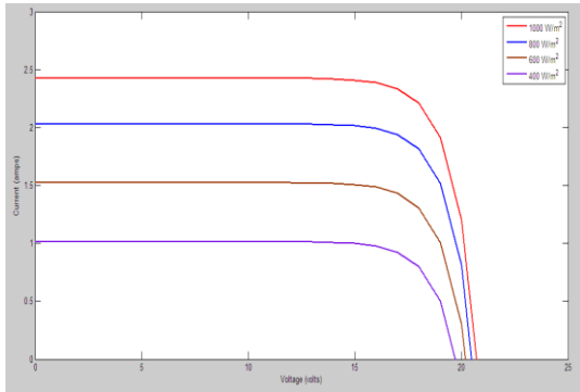
Figure 6 : I-V curves for different irradiance level Figure 7 : P-V curves for different irradiance level
