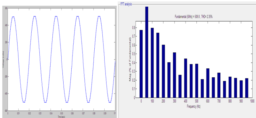
Figure 16: Output voltage waveform of Forty ninelevel MLI without buck-boost converter
