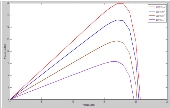
Figure 6 : I-V curves for different irradiance level Figure 7 : P-V curves for different irradiance level
