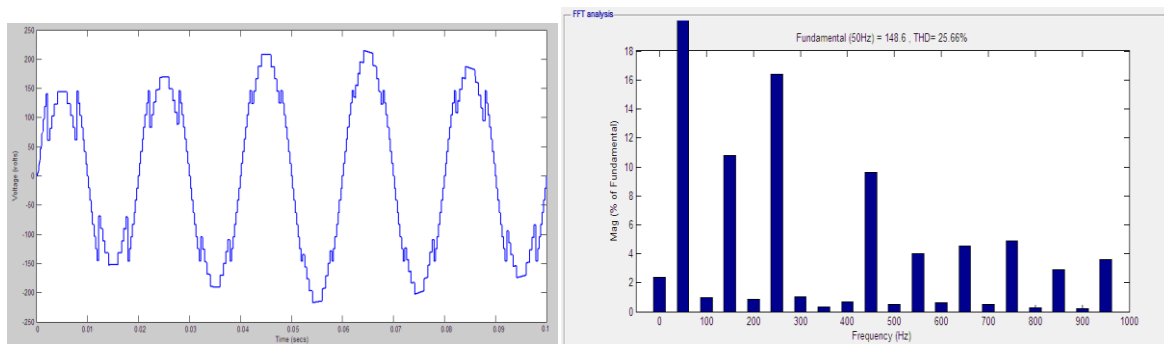
Figure 12: Output voltage waveform of Twenty five level MLI with buck-boost converter
