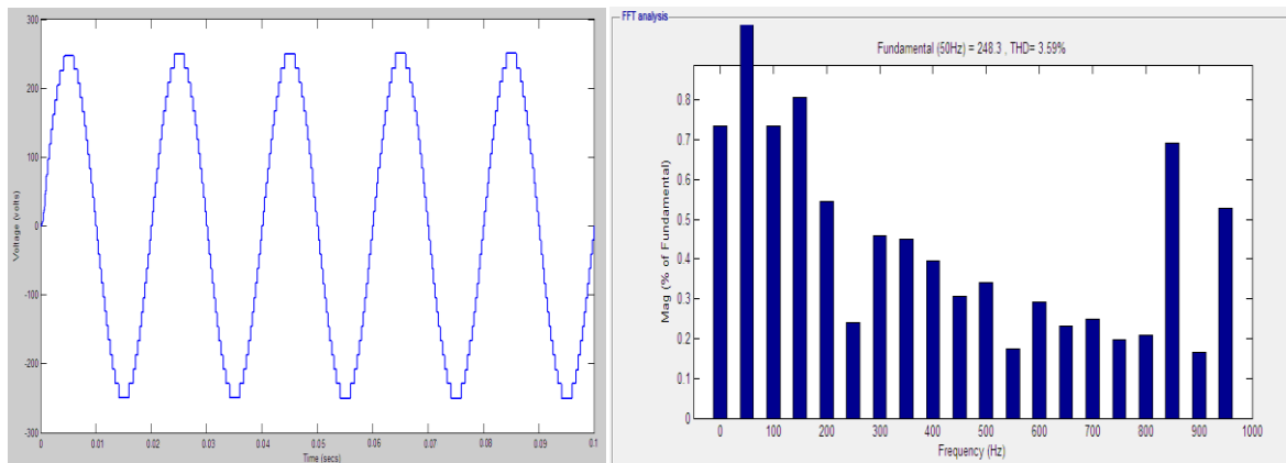
Figure 14: Output voltage waveform of Twenty five level MLI without buck-boost converter
