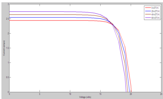
Figure 8 : I-V curves for different temperature level Figure 9: P-V curves for different temperature level
