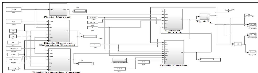
Figure 3: Simulink model of a PV module
