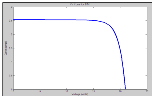
Figure 4 : I-V curve for STC
