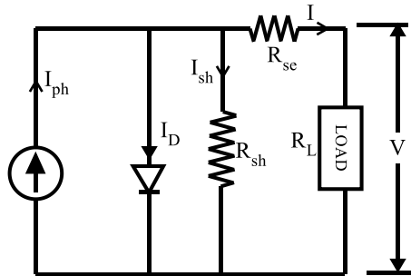
Figure 2.: Equivalent circuit of a solar cell
