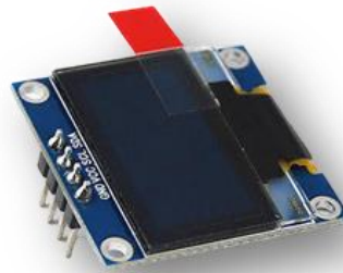
Fig. 7. Display (OLED)
