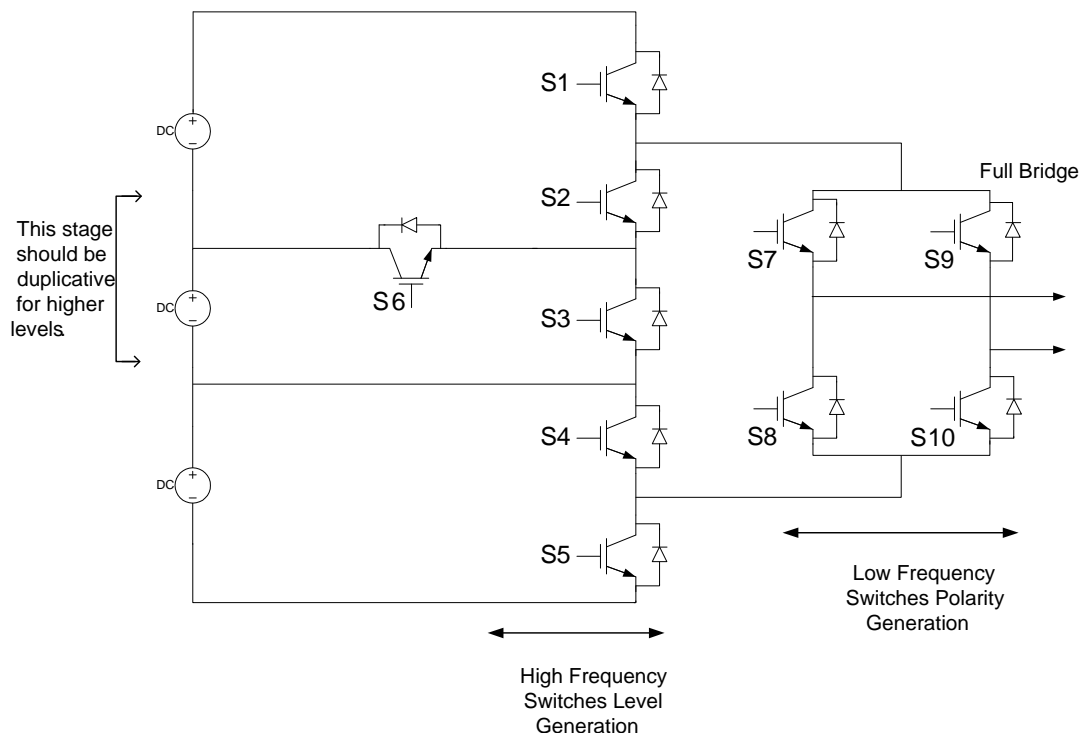
Fig. 1 Multi-level inverter using Reversing Voltage topology.
