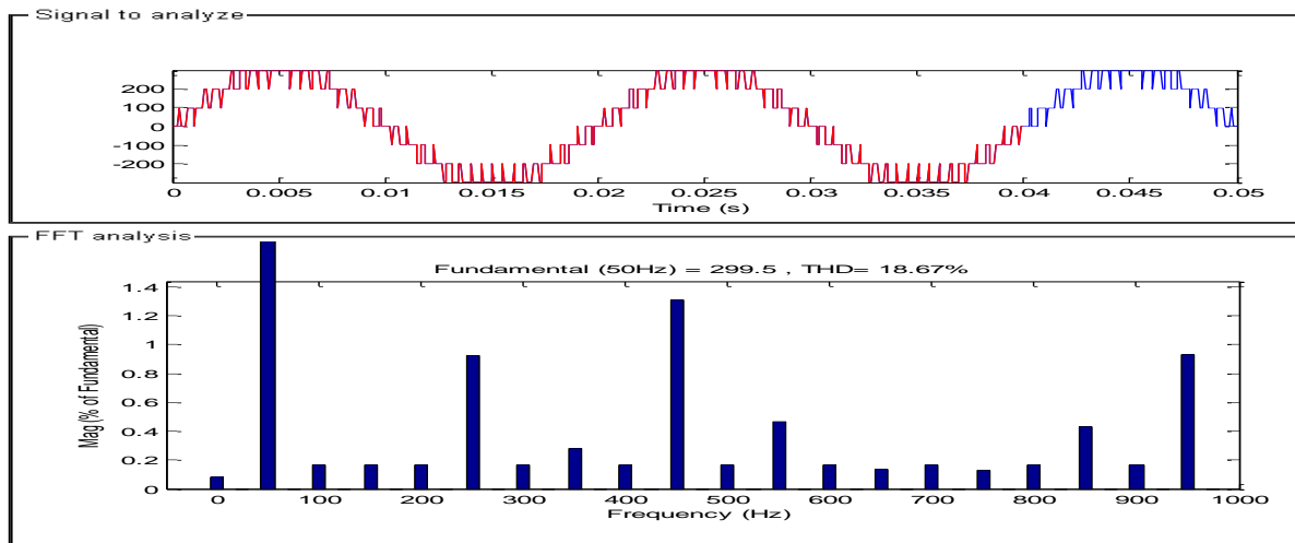
Fig. 8 Phase output voltage by PS PWM
