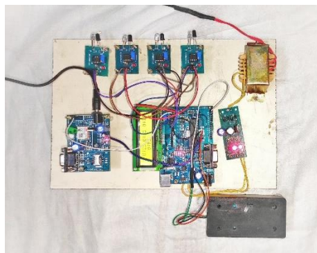
Fig.9.3 Receiver module
