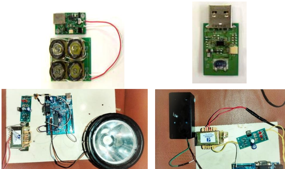
Fig.7.6 Transmitter
