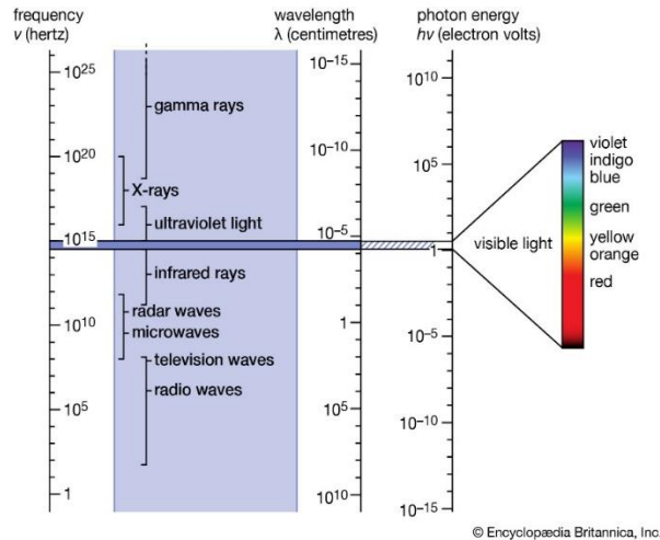
Fig.6.1 Electromagnetic Spectrum
