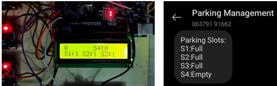
Fig.9.5 One parking slot is free
