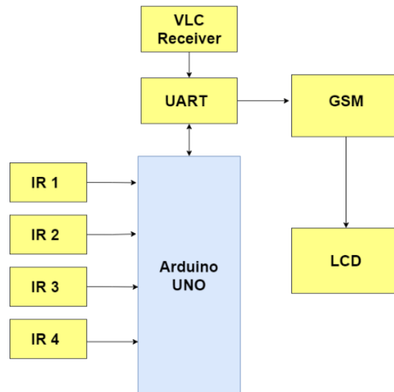
Fig.4.2 Block diagram of parking slot enquiry and detector module
