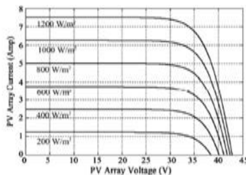
Fig.6 I-V characteristics of the solar PV array
