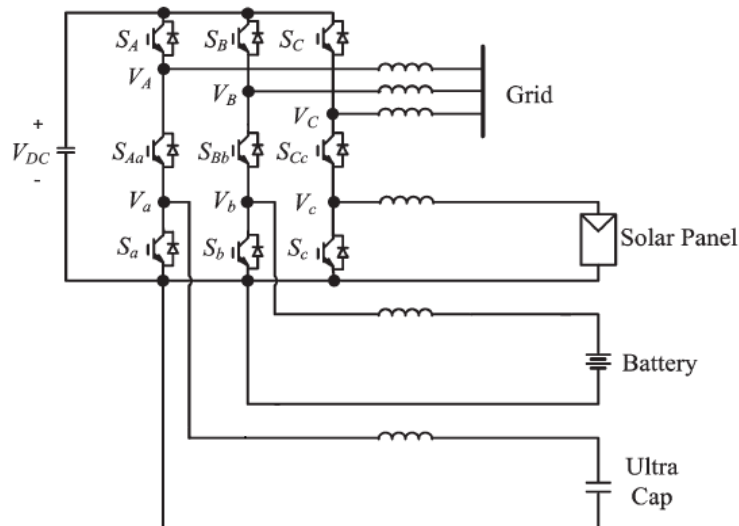
Fig. 3. Three phase Inverter having various Sources and Energy storage device
