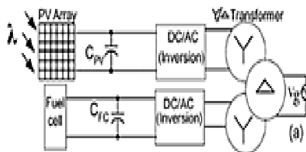
Fig.1 Conventional Topology for Two Multistage Inverters
