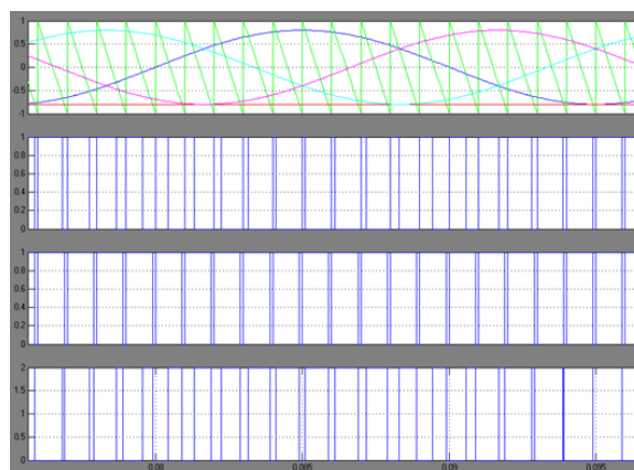
Fig.10 shows pulse pattern for switches.
