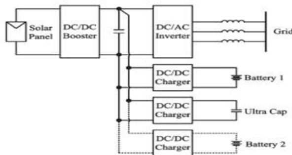
Fig.4 Block diagram of nonintegrated energy system
