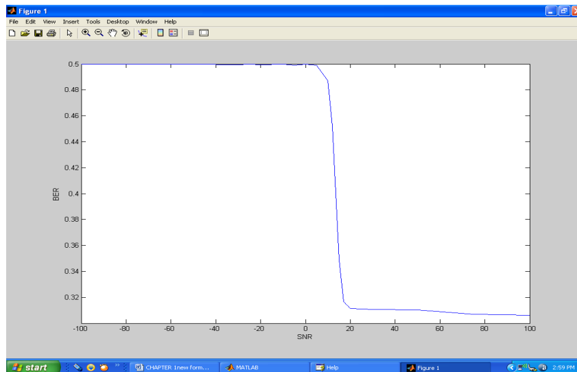
Figure 8. BER Plot of WiMAX system with RS Encoding
