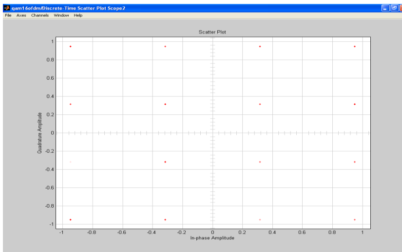
Figure 6. Constellation Diagram of Wimax System with 16 – QAM Modulation
