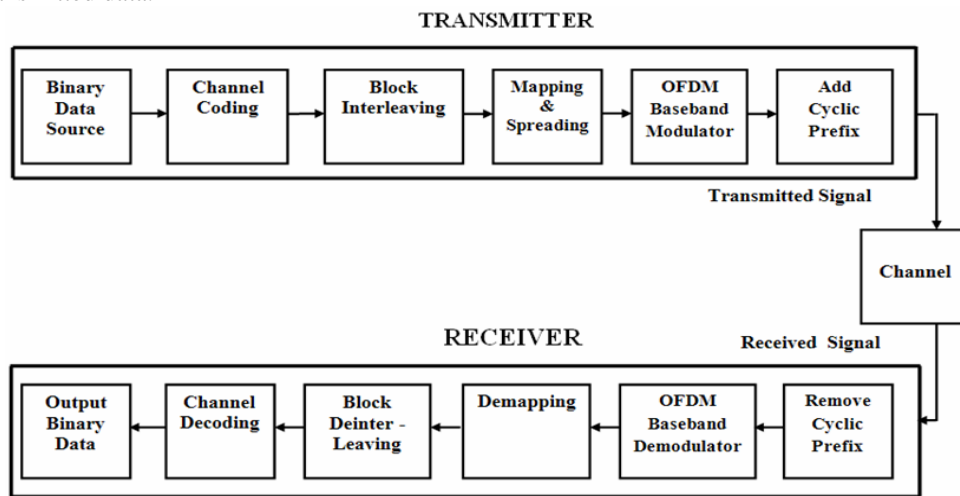
Figure 1: WiMax System.
