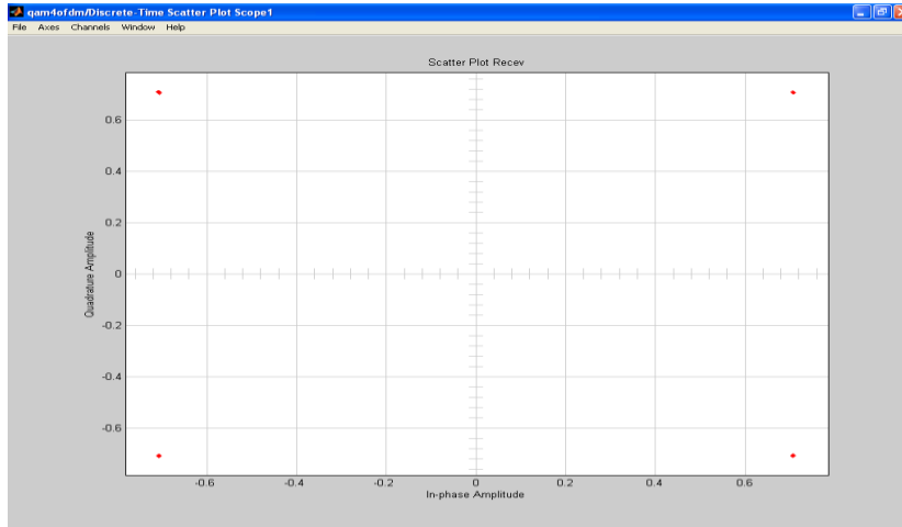
Figure 5. Constellation Diagram of Wimax System with 4 – QAM Modulation
