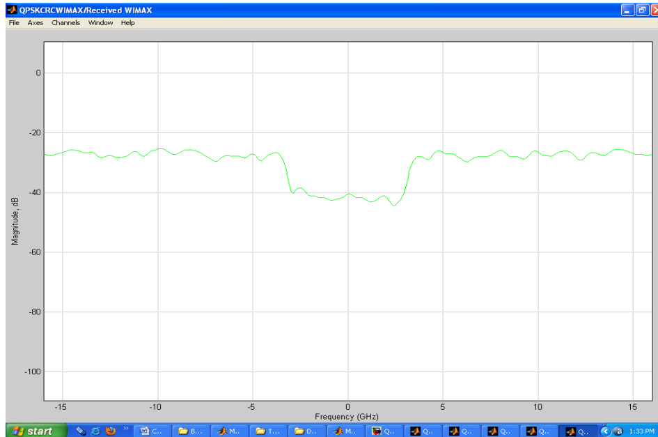
Figure 3. Received Signal of Wimax System
