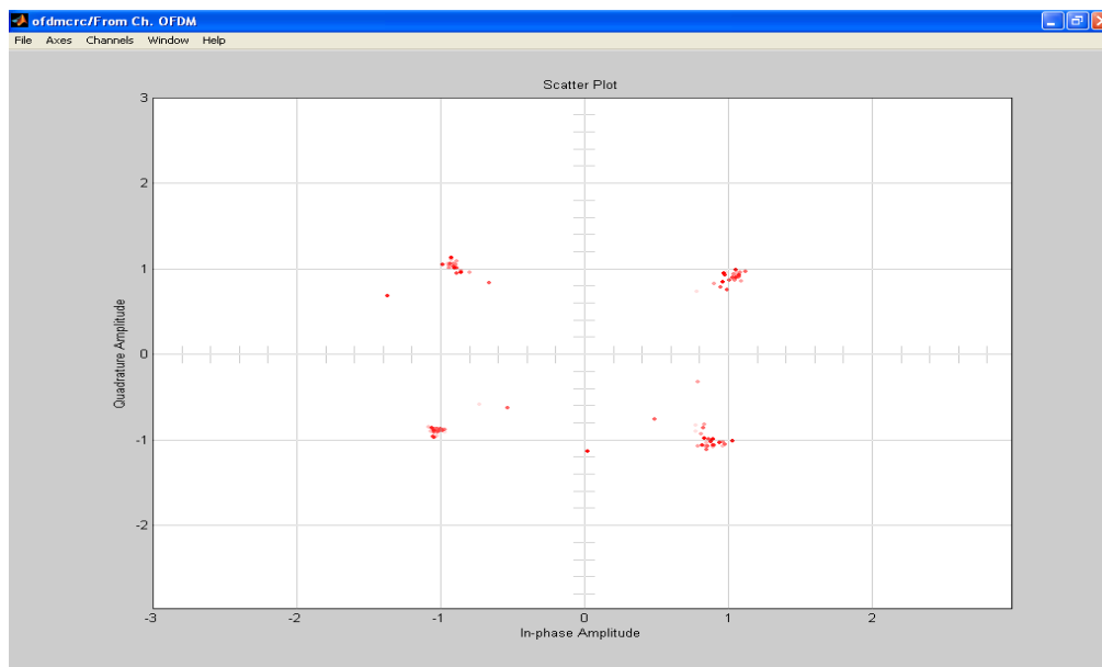
Figure 4. Constellation Diagram of Wimax System with QPSK Modulation.
