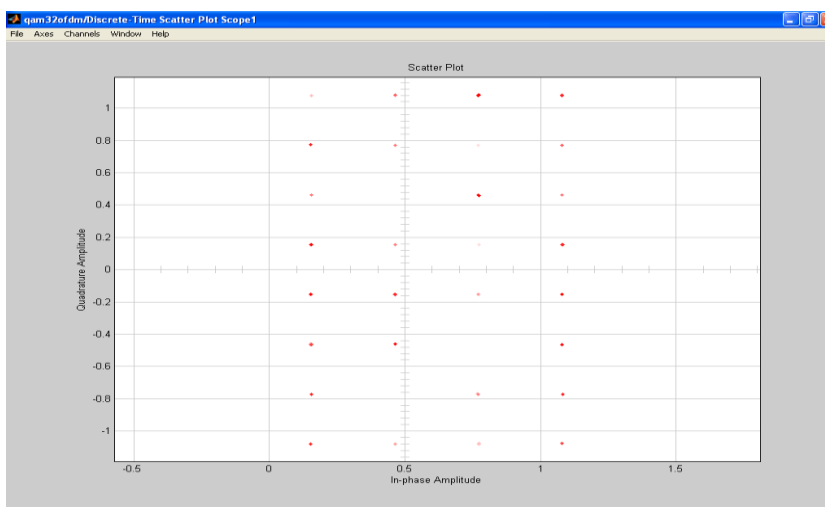
Figure 7. Constellation Diagram of Wimax System with 32 – QAM Modulation
