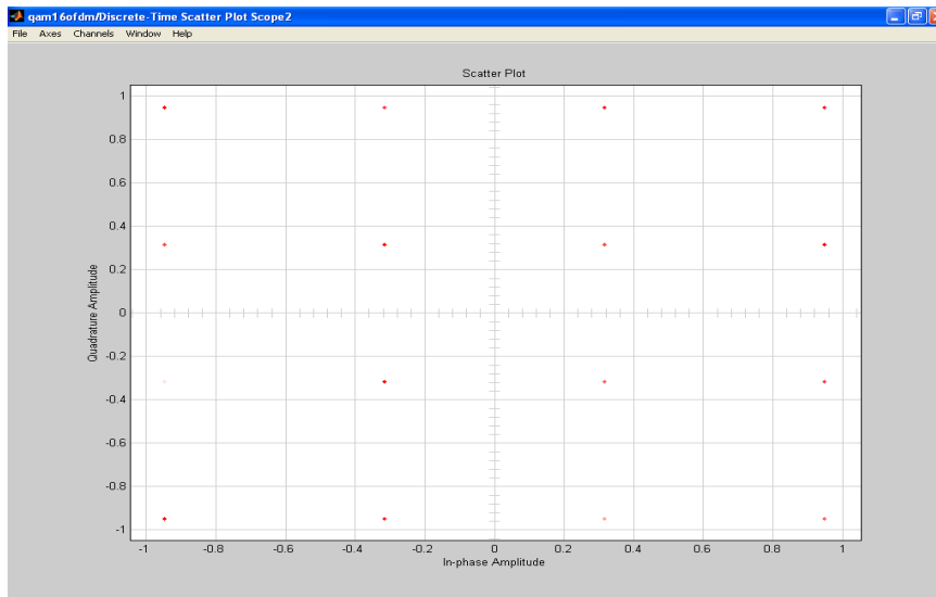
Figure 7. Constellation Diagram of OFDM System with 16 – QAM Modulation
