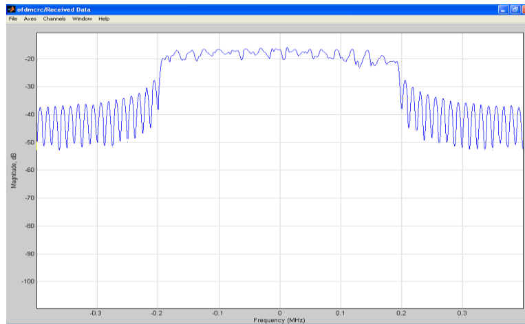
Figure 4. Received Signal of OFDM System
