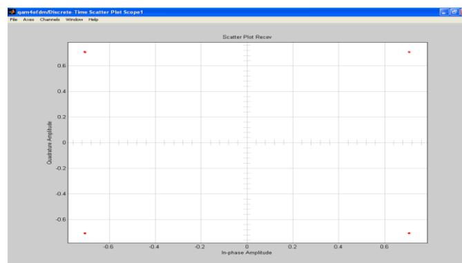
Figure 6. Constellation Diagram of OFDM System with 4 – QAM Modulation
