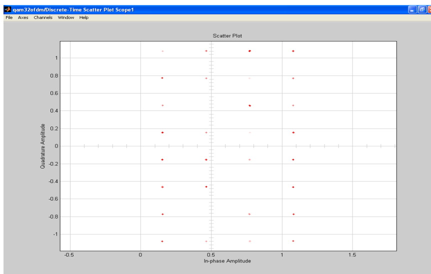
Figure 8. Constellation Diagram of OFDM System with 32 – QAM Modulation
