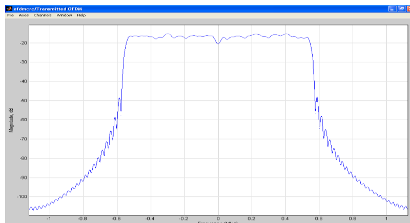
Figure 3. Transmitted Signal of OFDM System
