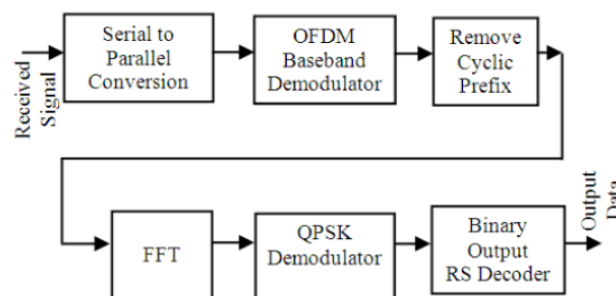
Figure 2. OFDM Receiver.
