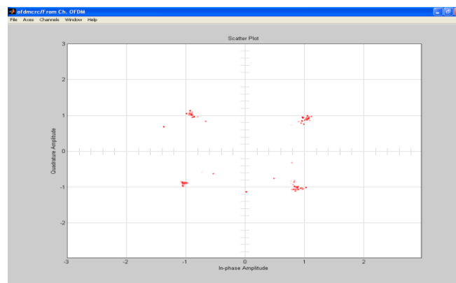
Figure 5. Constellation Diagram of OFDM System with QPSK Modulation
