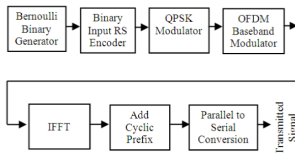
Figure 1. OFDM Transmitter.
