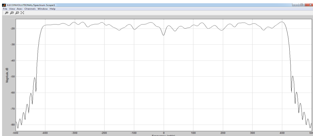
Figure 3. Transmitted Signal of HIPERLAN.
