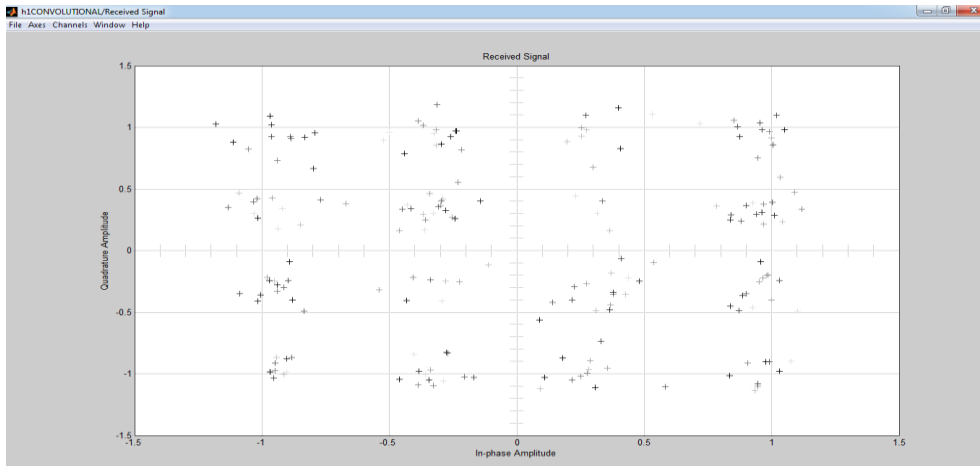
Figure 7. Constellation Plot of Received Signal of HIPERLAN.
