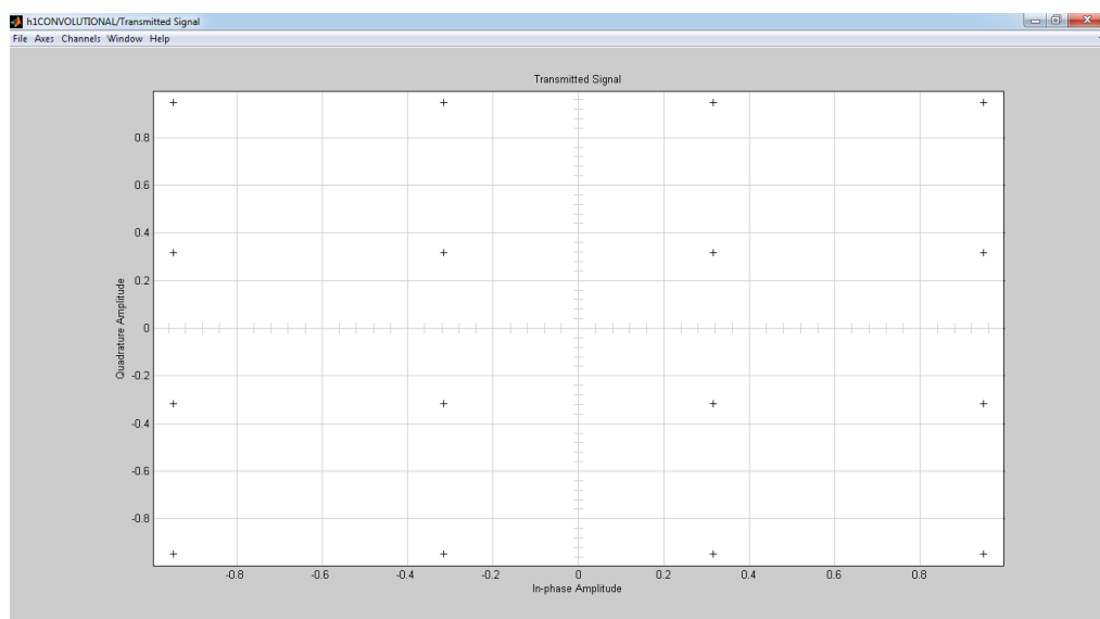
Figure 6. Constellation Plot of Transmitted Signal of HIPERLAN.
