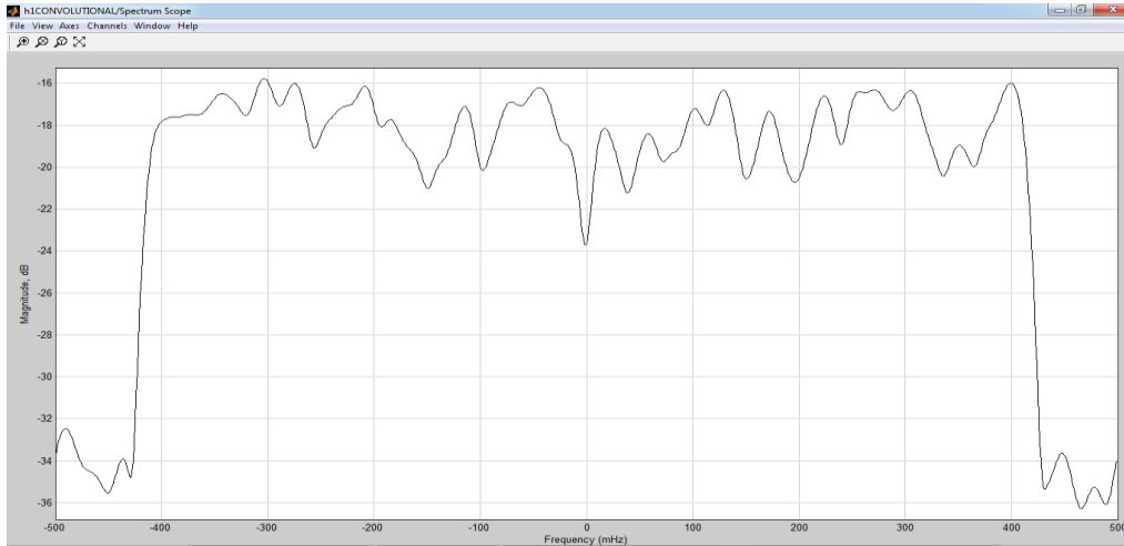
Figure 4. Received Signal of HIPERLAN.
