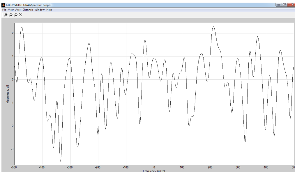
Figure 5. Received Signal of HIPERLAN After OFDM Modulator.
