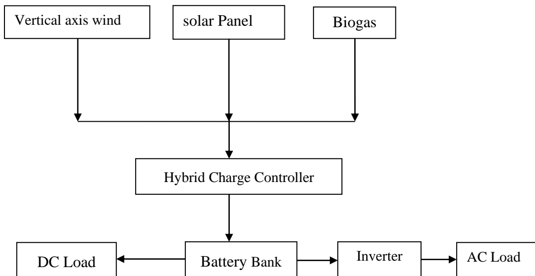
Fig. 1 A sample graph
