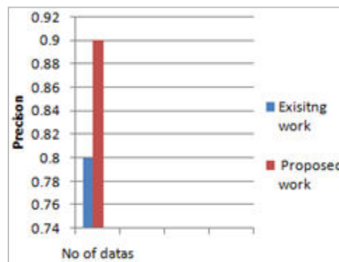
Fig. 1 Precision comparison
