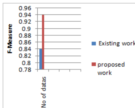
Fig. 3 F-Measure comparison
