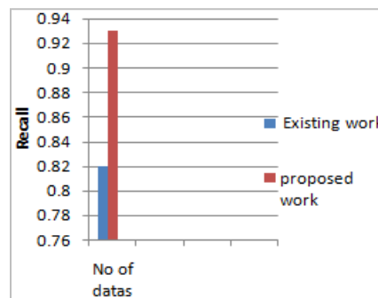
Fig. 2 Recall Comparison
