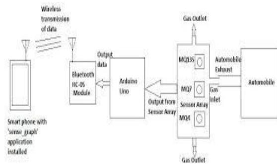
Fig .4 General block diagram of electronic nose
