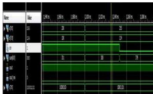
Fig. 7 Simulated output of CI-CSKA Structure
