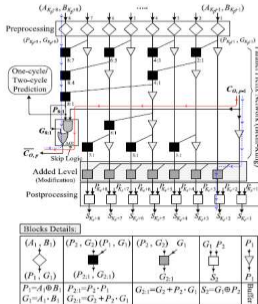
Fig. 5. Internal structure of the p th stage of the hybrid variable latency CSKA.
