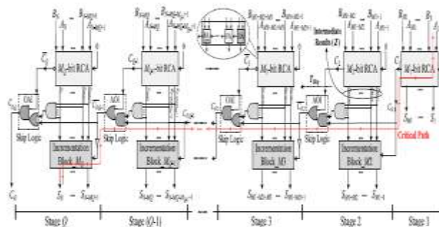
Fig. 2. Proposed CI-CSKA structure
