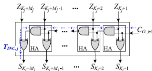
Fig. 3. Internal Structure of Incrementation Block
