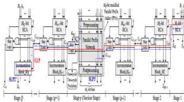
Fig. 4. Structure of the hybrid variable latency CSKA
