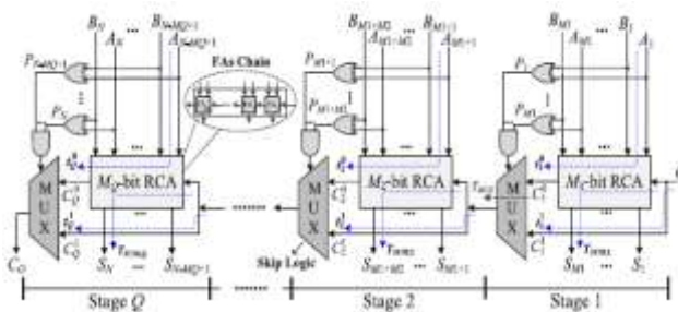
Fig. 1. Conventional structure of the CSKA
