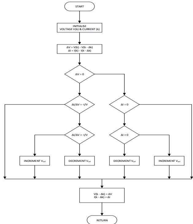
Fig 8: Flow Chart Incremental Conductance
