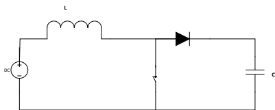
Fig 5: Boost Converter
