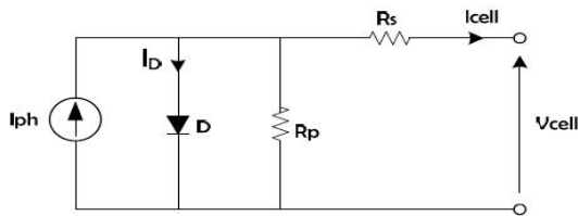
Fig 1: Equivalent Circuit
