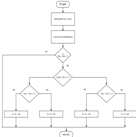
Fig 7: Flow Chart P&O
