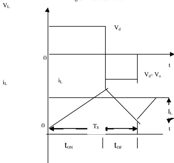
Fig 6: Wave Forms
