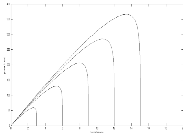
Fig 3: PV Characteristics
