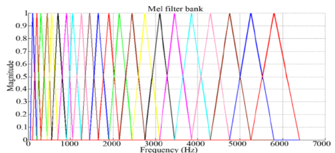
Figure 2. Mel filter bank.
