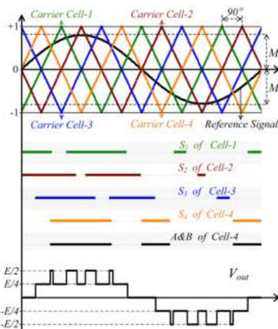
Fig 3. Switching pattern based on the PS-PWM, states of the power switches and switched output voltage of a 4-cell-five-level FCMC.
