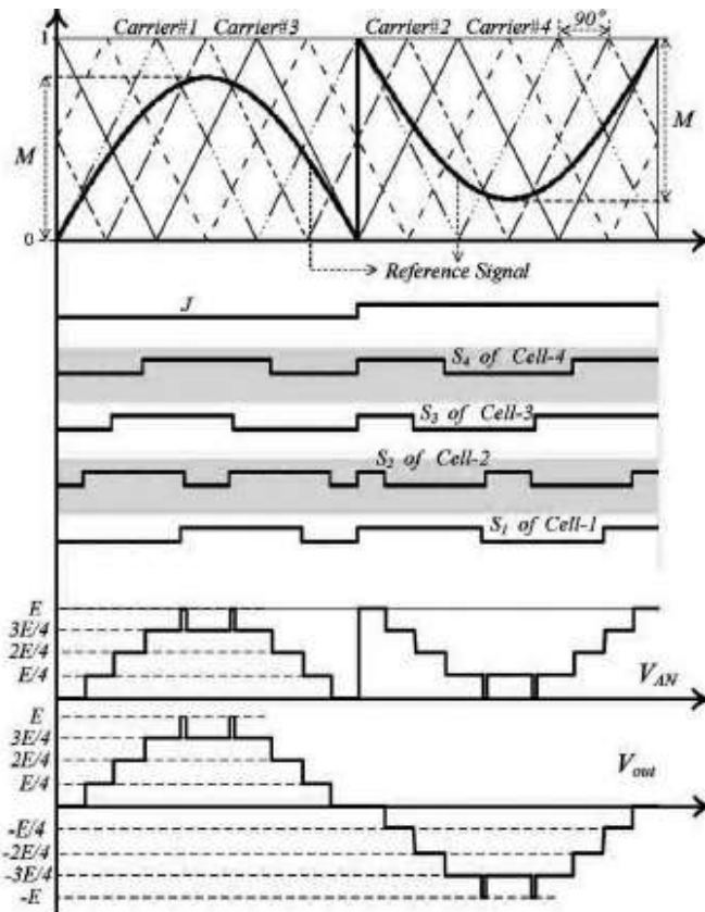
Fig 4. Control Strategy for 4-cell 9-level DFCM Converter
