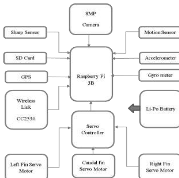
Figure 1: Block Diagram
