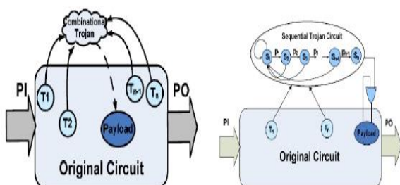
Figure 3: Illustration of a combinational and sequential Trojan (Source: [7])
