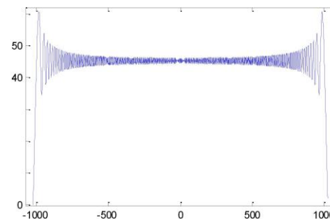
Fig.4. Spectrum of the ZC sequence with FFT shift.
