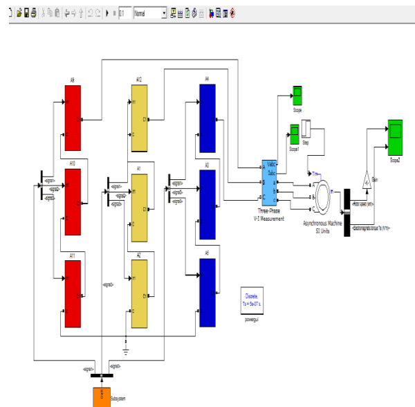
Fig.1 Seven Level Inverter fed Induction Motor Drive
