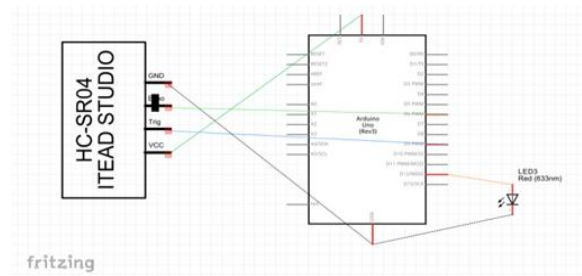
Fig5 Schematic diagram sensor based accident prevention system.
