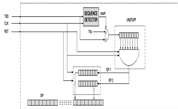
Fig. 6 HDLC receiver
