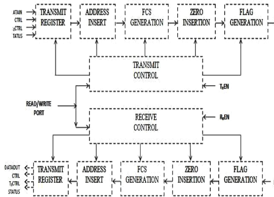
Fig. 7 HDLC transceiver
