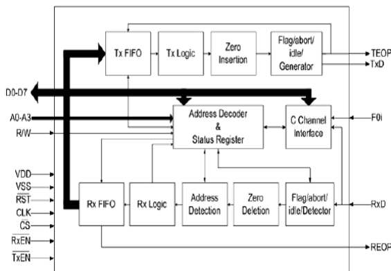
Fig. 2 HDLC controller
