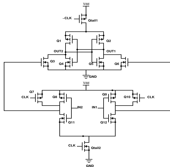
Fig.4. Schematic diagram of the optimised double-tail dynamic comparator
