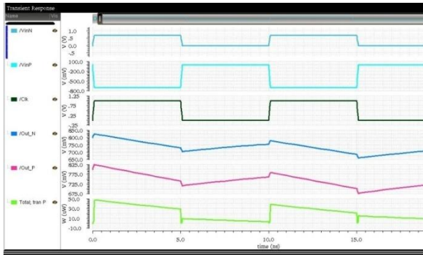
Fig.3. Transient simulations of the conventional double-tail dynamic comparator for input voltage difference of \Delta V_d = 0.7 V, and V_{DD} = 0.8 V.
