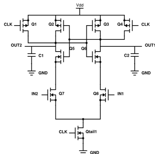
Fig 1.Schematic diagram of the conventional dynamic comparator
