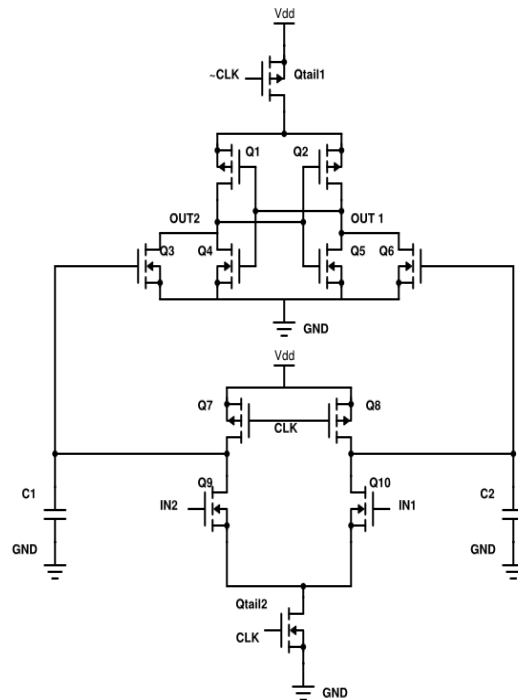
Fig. 3. Schematic diagram of the conventional double-tail dynamic comparator
