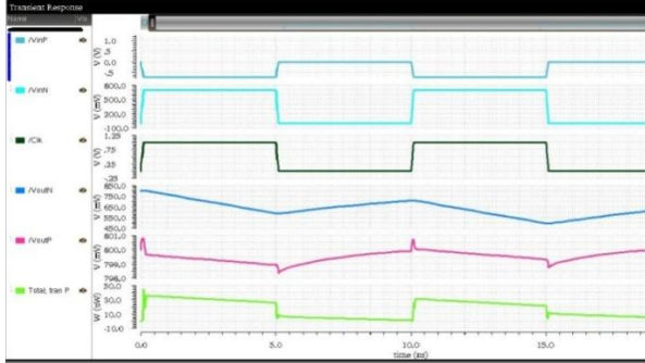
Fig.2. Transient simulations of the conventional dynamic comparator for input voltage difference of \Delta V_d = 0.7 V, and V_{DD} = 0.8 V.
