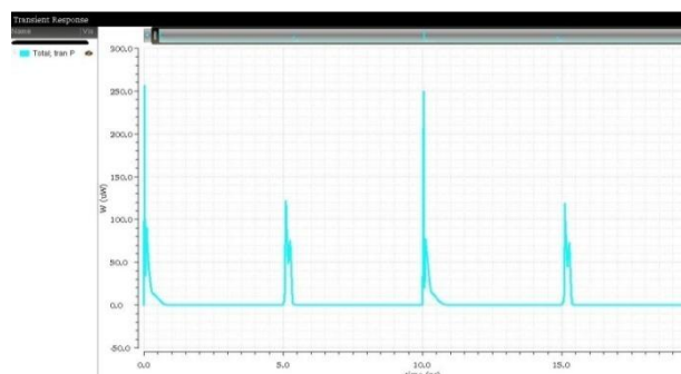
Fig.4. power dissipation of the proposed optimised double-tail dynamic comparator
