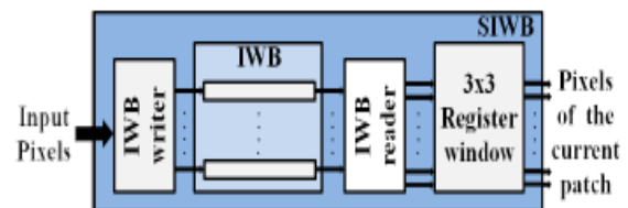
Figure 6: SIWB Internal architecture
