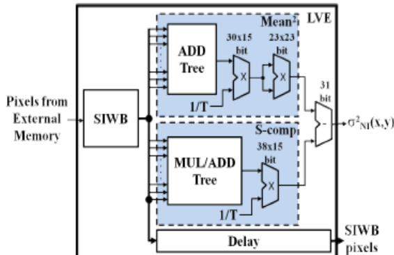
Figure 7: LVE Internal architecture
