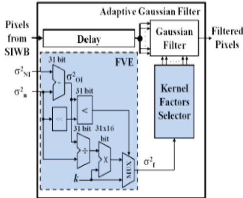
Figure 8: Adaptive Gaussian Internal architecture
