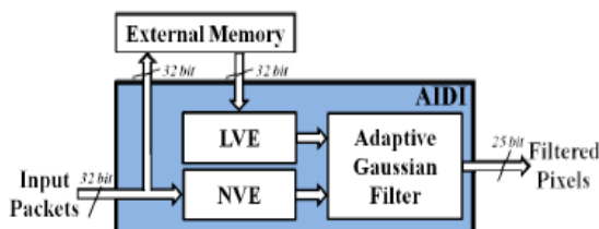
Figure 1: AIDI Internal architecture
