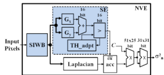
Figure 5: NVE Internal architecture
