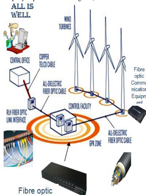
Fig.6 Typical Fibre Optic Network in Onshore Wind Farm Source: http://www.fibreopticlink.com/Industry_Solutions/Wind_Energy.html
