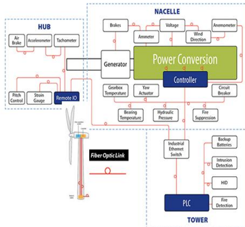
Fig.5. Fibre Optic Control Networking in a wind turbine. Source: http://www.firecomms.com/applications-renewable_energy.html
