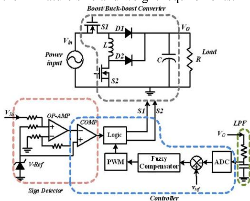
Fig. 2. Control circuit for the proposed converter.
