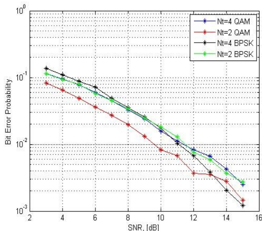
FIG 9 BER PERFORMANCE FOR DIFFERENT ANTENNAS USING QAM AND BPSK MODULATION SCHEMES
