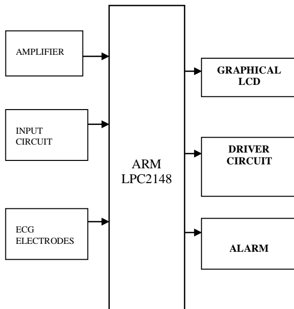
FIG.1.Proposed Block Diagram
