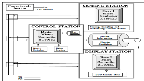
Figure 2.1 Block Diagram of Master/Slave communication.
