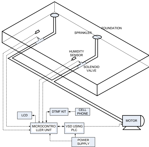
Fig. 1 Demonstration Prototype Layout
